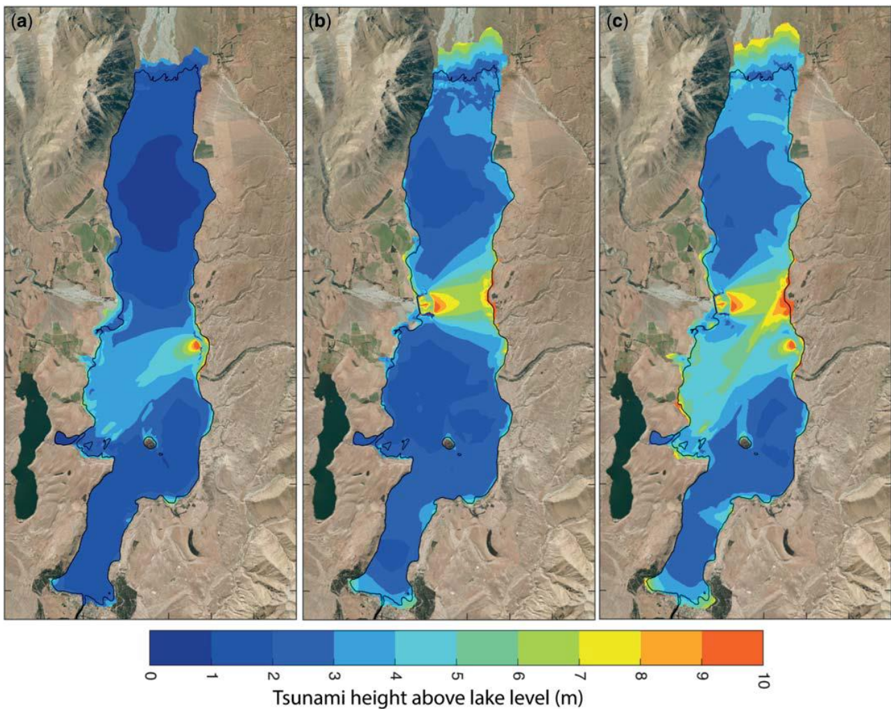
Figure 23: Scenario modelling results for (a) validation scenario V01; (b) validation scenario V02 and (c) combined modelling result for both scenarios occurring simultaneously (Mountjoy et al., 2018).
