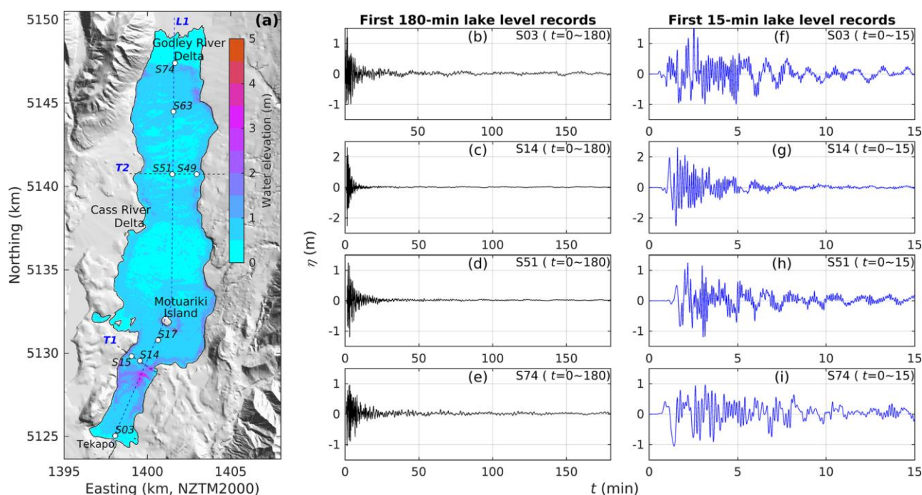
Figure 22: a) Spatial distribution of modelled maximum water elevation in Lake Tekapo. Colour scale indicates water elevation in metres above normal (Wang et al., 2020).
